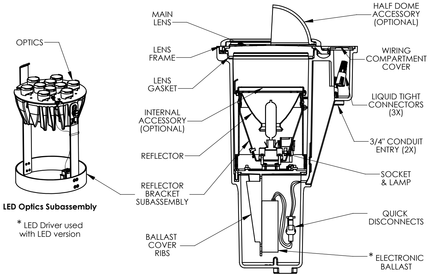
T6 HID Fixture Shown
