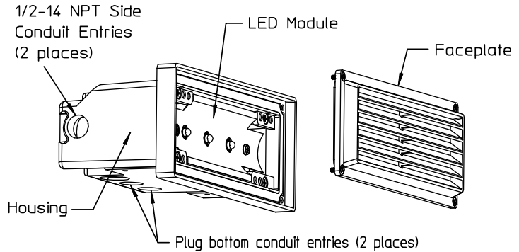
Figure 1. Loosen 4 screws to remove faceplate.
