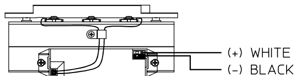
Figure 3. Connect supply wires to LED driver.
